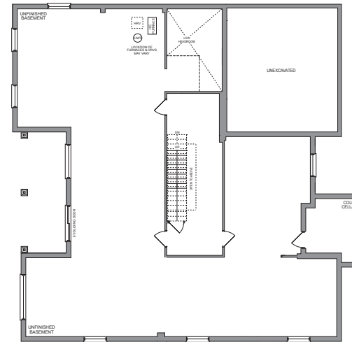
OPT. WALK-OUT BASEMENT - (INCLUDES 308 SQ. FT. OF FINISHED BASEMENT) ELEVATION A
