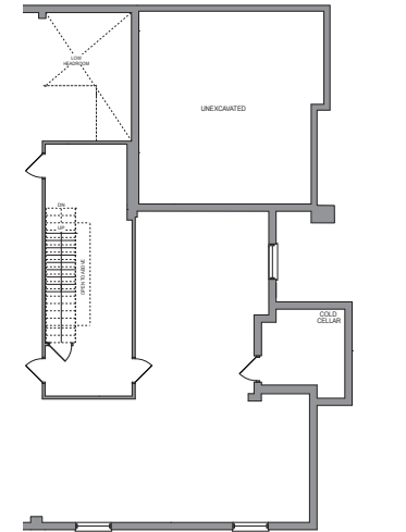
WALK-OUT BASEMENT - UNFINISHED (INCLUDES 308 SQ. FT. OF FINISHED BASEMENT) ELEVATION B
