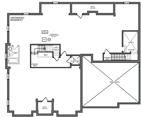
BASEMENT
